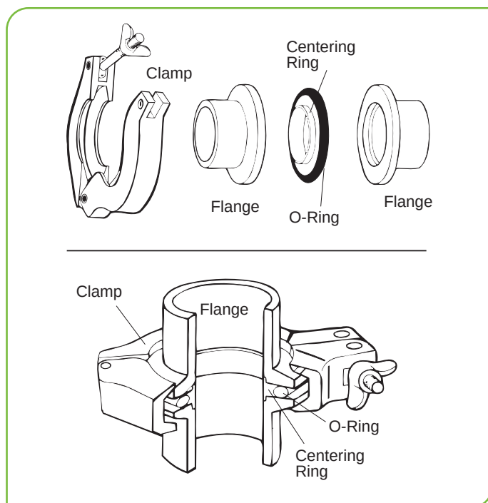
Figure 2 — Component Assembly
