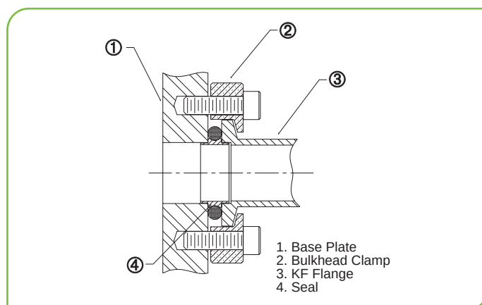
Figure 4 — Bulkhead Clamp
