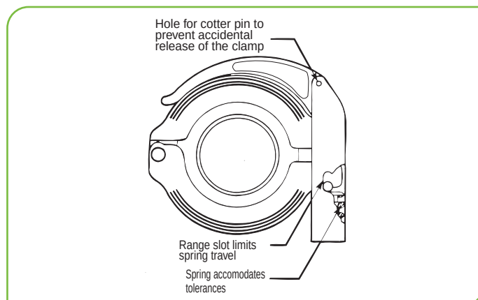
Figure 3 — Toggle Clamp
