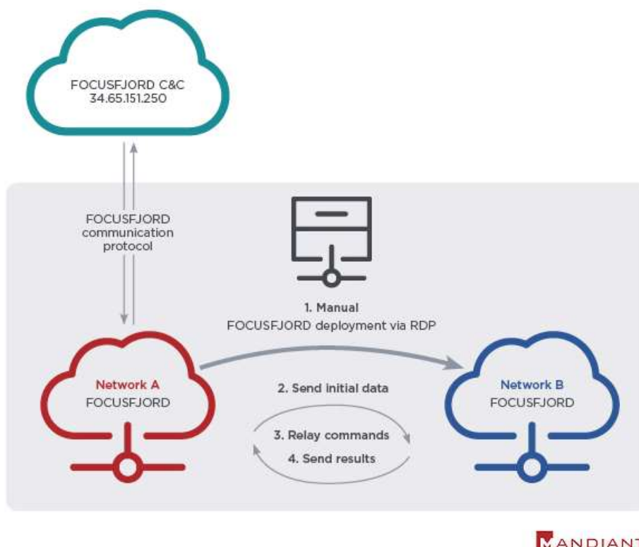
Figure 22 - Two FOCUSFJORD samples configured to proxy C&C traffic
